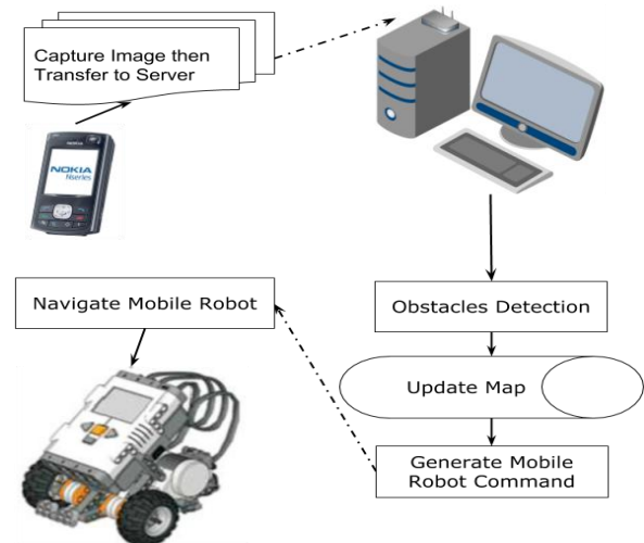
Figure 3: Remote-brained LEGO Robot operations
